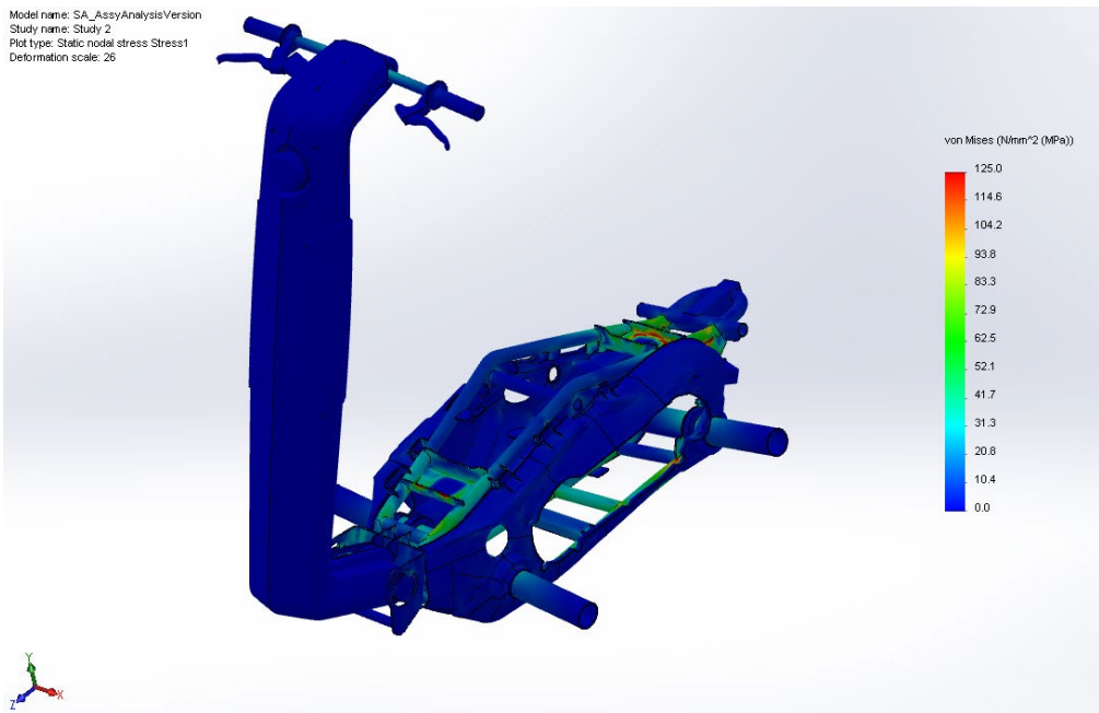
Structural Analysis provides Stress distribution to identify critical areas
